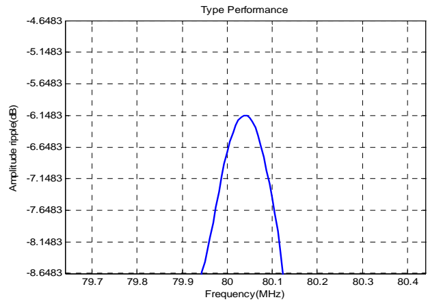
Passband Respond
