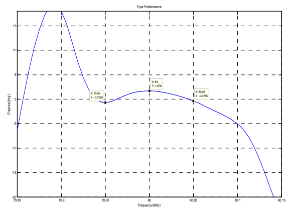
Phase Linearity(f0±0.05MHz)
