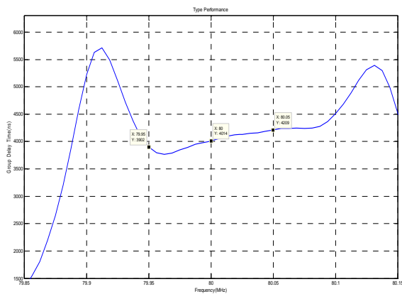
Group Delay Variation(f0±0.05MHz)
