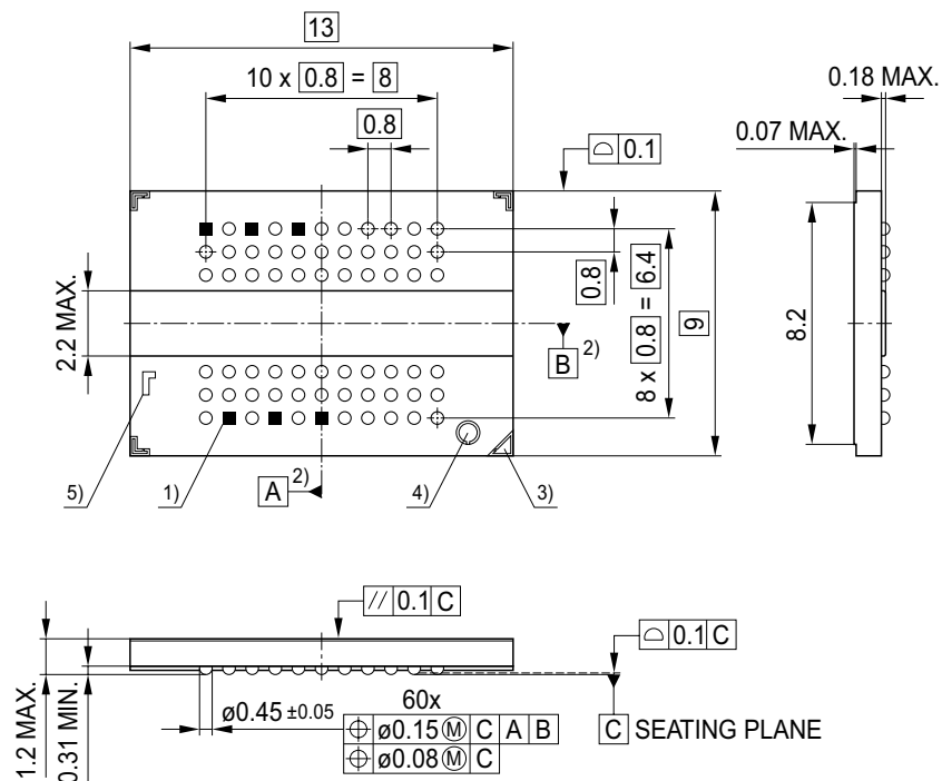
FIGURE 11 Package Outline PG-TFBGA-60
