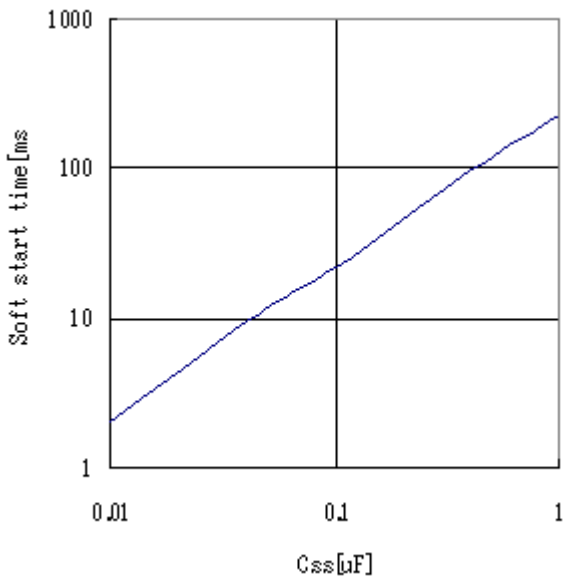
Figure 12. Soft Start Time
