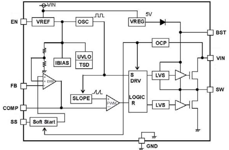
Figure 3. Block Diagram
