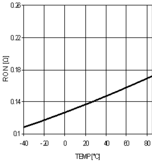
Figure 8. Hi,Low-Side On-resistance
