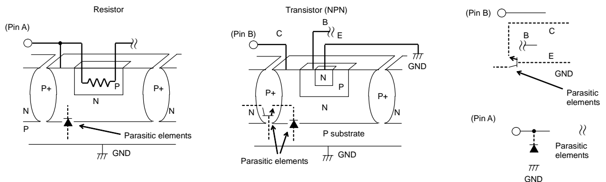
Figure 29. Example of a Simple Monolithic IC Architecture
