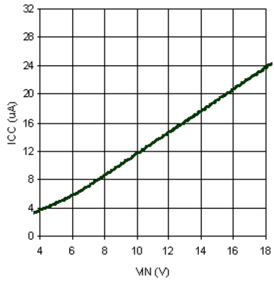
Figure 5. Stand by current (IC not active)
