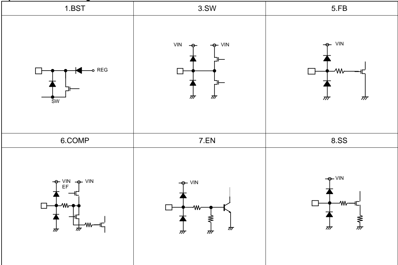
Figure 28. I/O Equivalent Circuit
