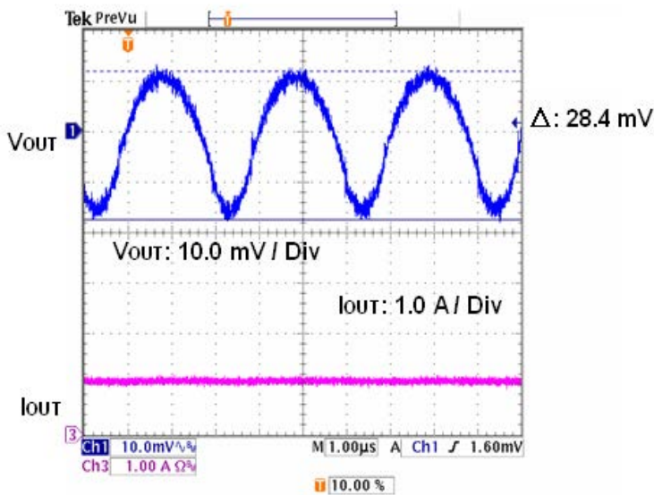
Figure 14. Output Ripple Voltage (VIN= 12V VOUT= 3.3V L= 10μH Cout =22μF I out= 1.0A )
