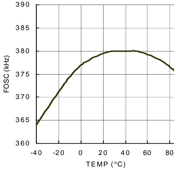
Figure 9. Operating Frequency
