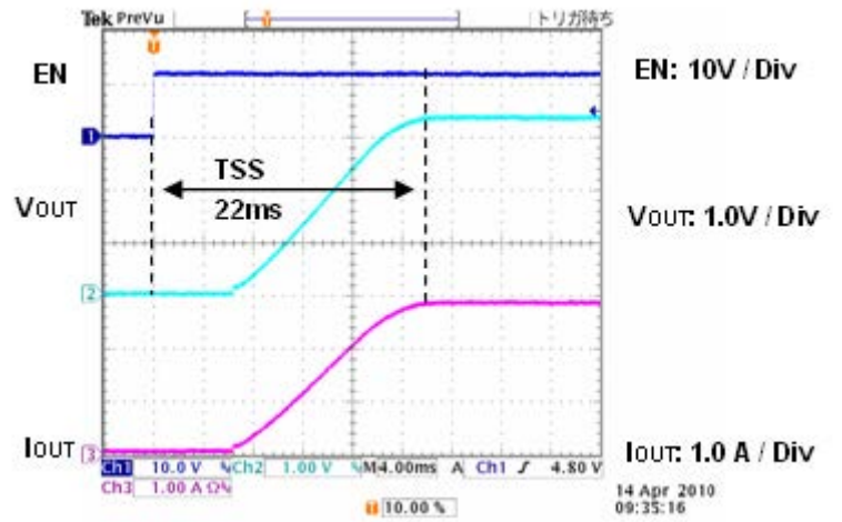
Figure 17. Start Up waveform (VIN= 12V VOUT= 3.3V L= 10μH CSS= 0.1μF)
