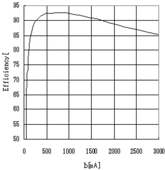
Figure 10. STEP Down Efficiency (VIN= 12V VOUT= 3.3V L=10μH)
