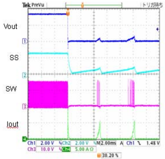
Figure 11. OverCurrent Protection (Vout is shorted to GND)
