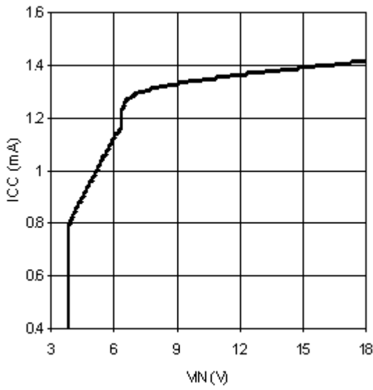
Figure 4. Circuit Current (No switching)
