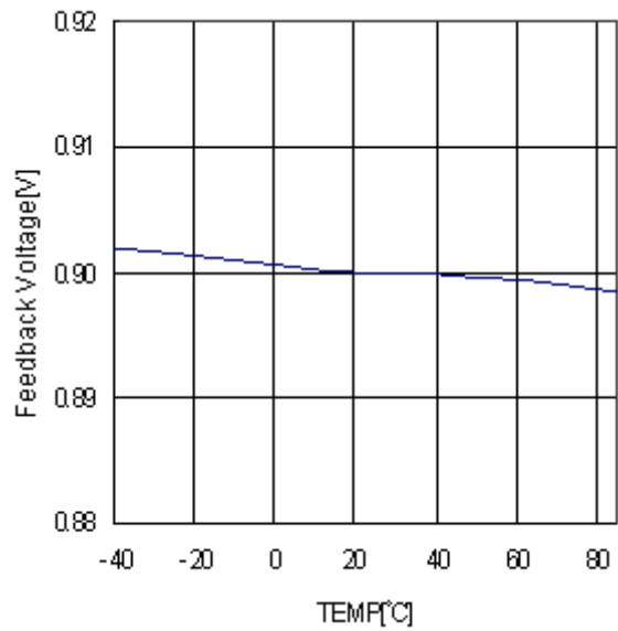
Figure 7. Feedback voltage
