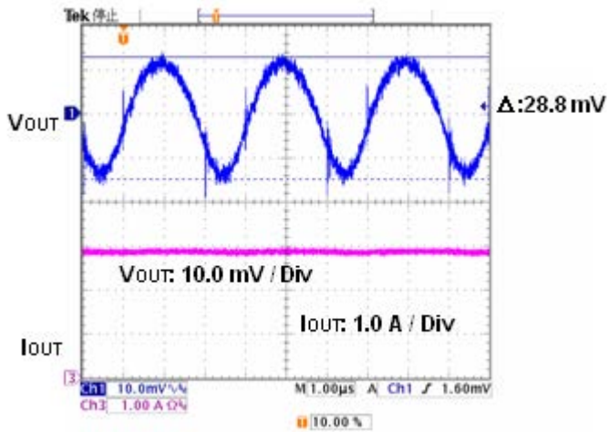
Figure 16. Output Ripple Voltage (VIN= 12V VOUT= 3.3V L= 10μH Cout =22μF I out= 3.0A)
