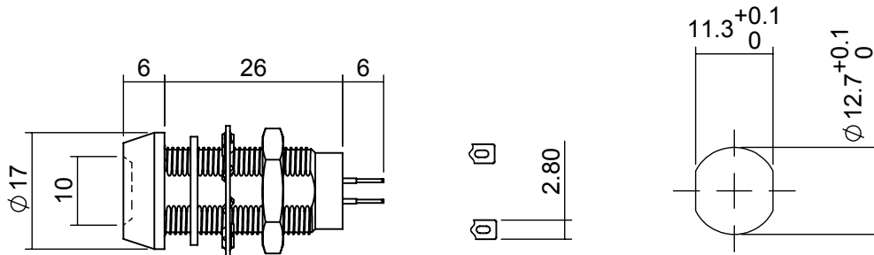
Mounting Hole
