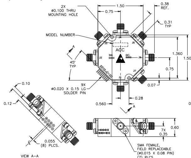
OUTLINE CASE STYLE S6
