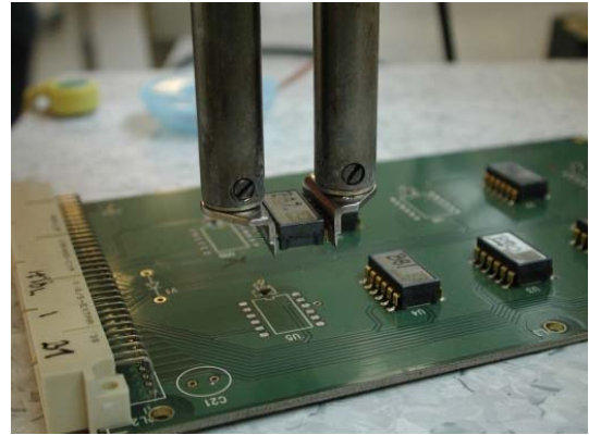
Figure 14. Immediately after solder melting, component is lifted.
