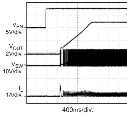
Startup Through EN I_{OUT} = 0.1A
