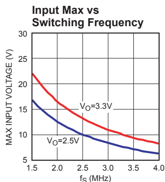
Figure 2—Recommended Input vs. f_s
