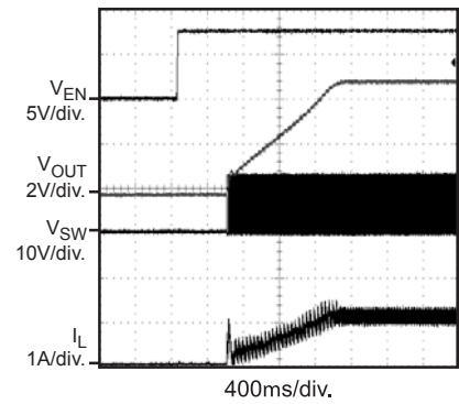
Startup Through EN I_{OUT} = 1A
