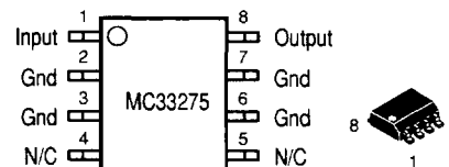
D SUFFIX PLASTIC PACKAGE CASE 751-06 (SOP-8)
