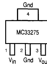
ST SUFFIX PLASTIC PACKAGE CASE 318E-04 (SOT-223)
