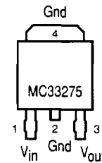
DT SUFFIX PLASTIC PACKAGE CASE 369A (DPAK)
