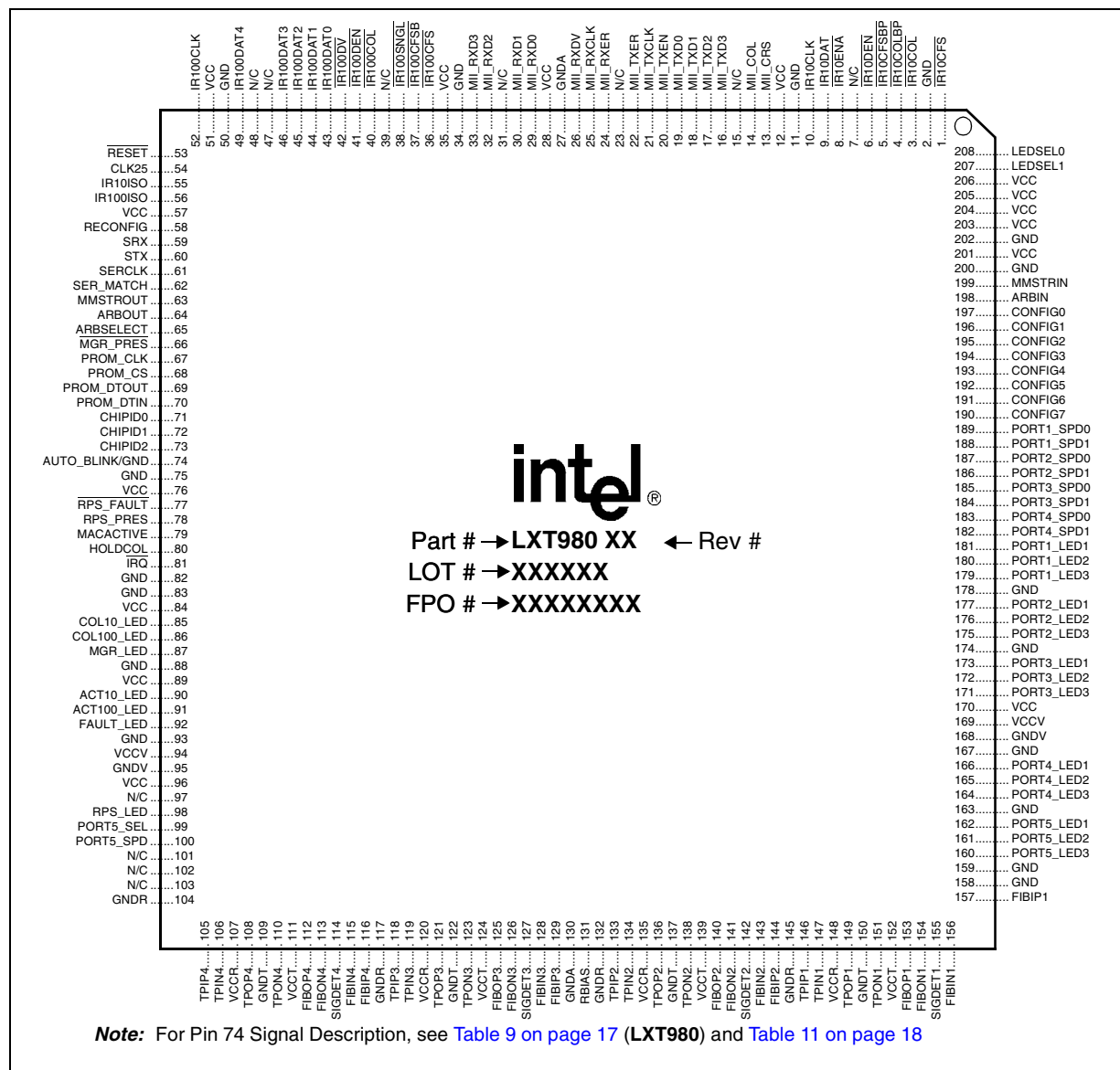
Figure 2. Pin Assignments
