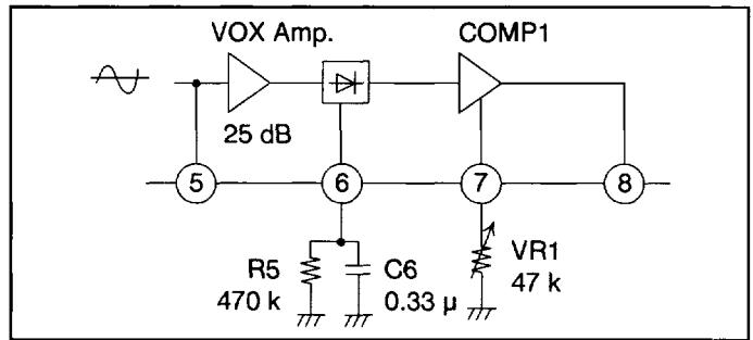
Figure 4 VOX Circuit
