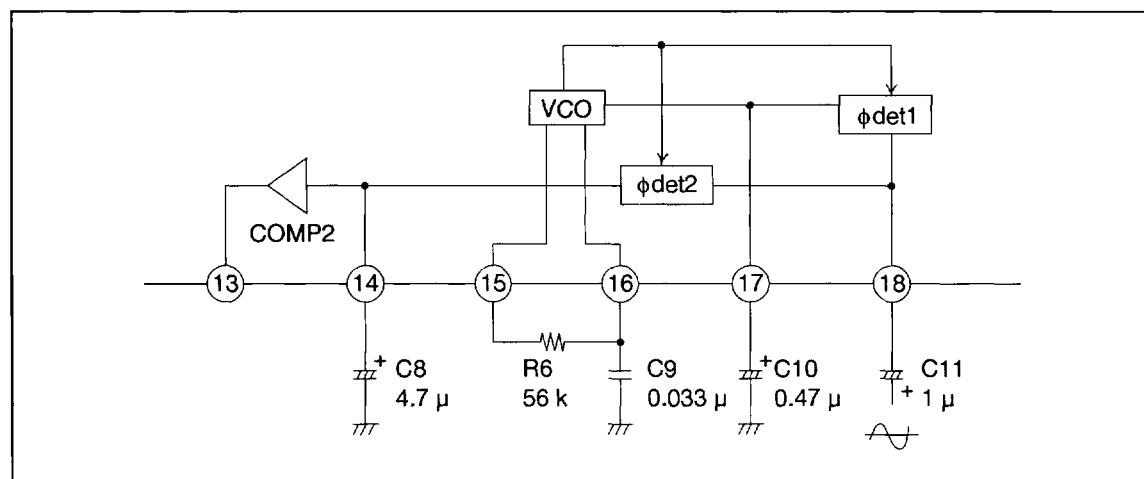
Figure 9 Busy Tone Detection Circuit
