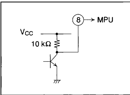
Figure 3 VOX Comparator Output
