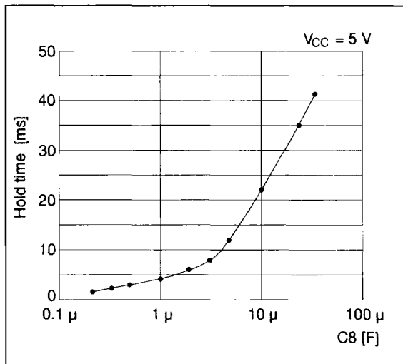
Figure 16 Hold Time vs. C8
