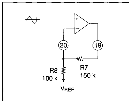
Figure 7 Amp 1 Circuit Diagram
