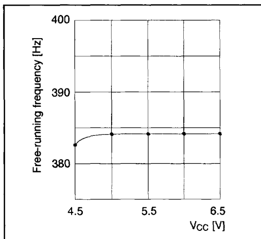
Figure 10 Free-Running Frequency vs. VCC
