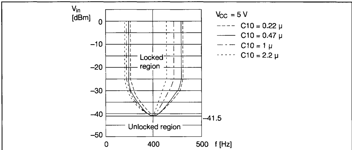
Figure 14 Input Level and Frequency vs. Busy Tone Frequency
