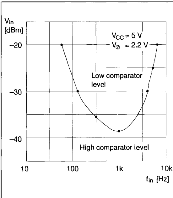
Figure 5 Input Level and Frequency vs. VOX Characteristic
