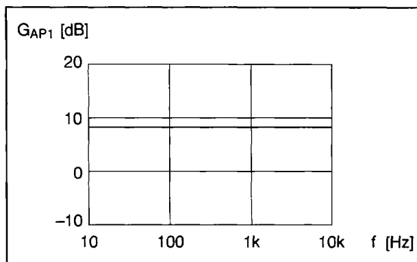
Figure 8 Amp 1 Gain vs. Frequency Characteristic
