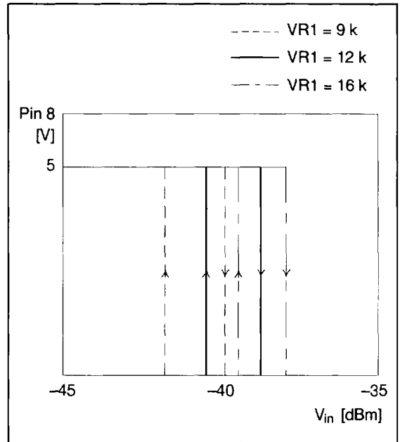
Figure 6 VOX Characteristic
