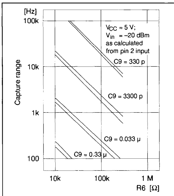
Figure 13 Capture Range vs. R6 & C9
