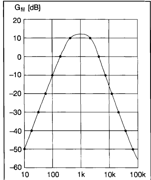
Figure 2 Filter Amplifier Gain vs. Frequency Characteristics
