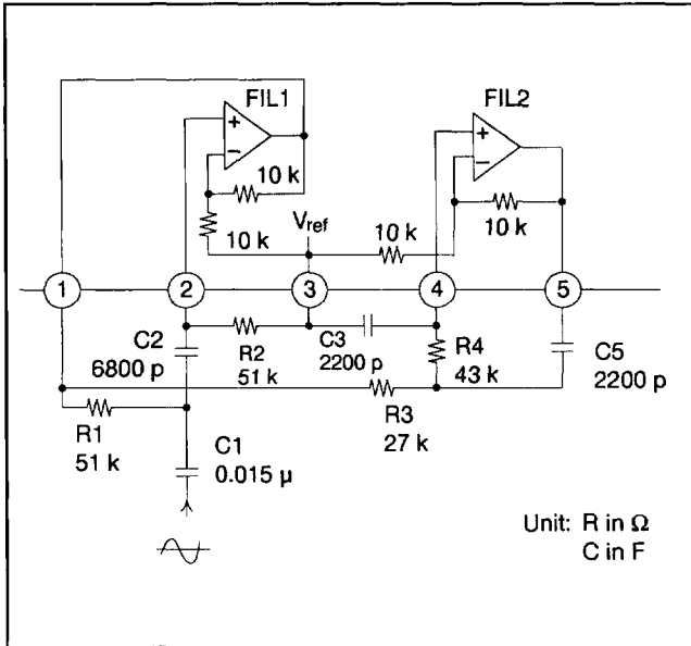
Figure 1 Filter Amplifier Circuit
