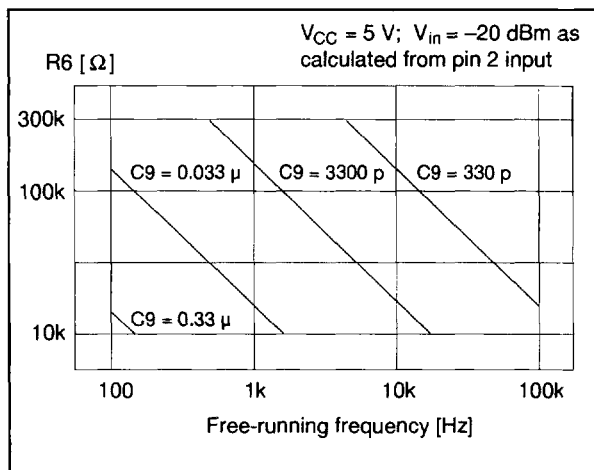
Figure 11 R6 & C9 vs. Free-Running Frequency
