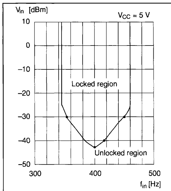
Figure 12 Input Level and Frequency vs. Busy Tone Frequency Characteristics
