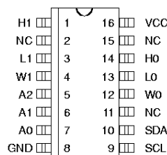
DS1803Z 16-PIN SOIC (150 MIL) DS1803 16-PIN DIP (300 MIL) See Mech. Drawings Section
