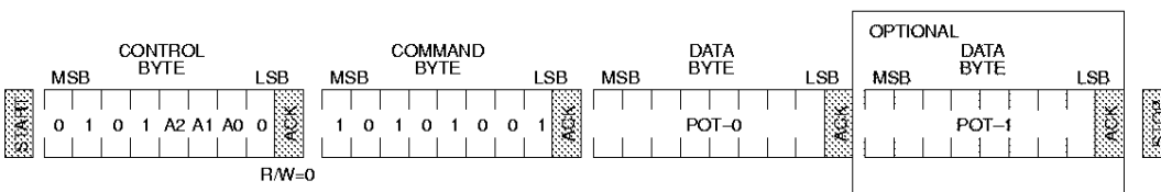
2-WIRE WRITE PROTOCOLS Figure 5
