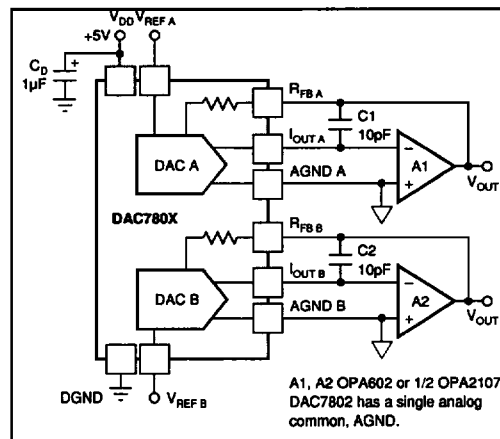
FIGURE 3. Unipolar Configuration.
