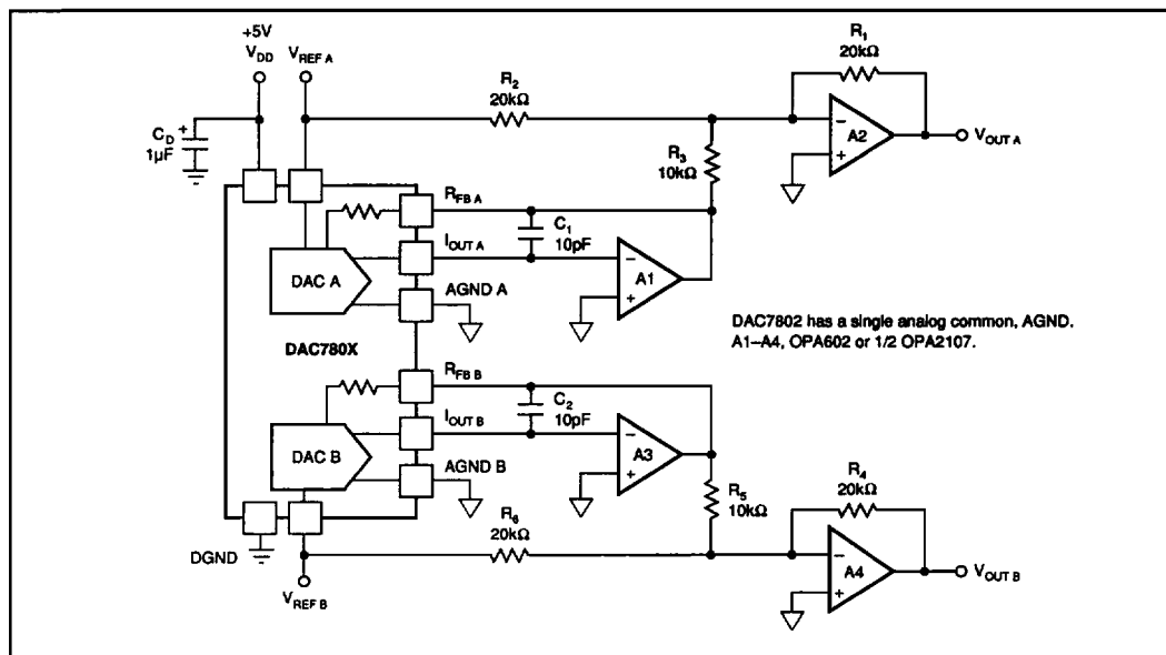
FIGURE 5. Bipolar Configuration.
