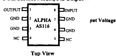
8-Pin Surface Mount, Fix Output
