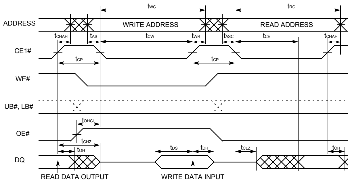
Figure 44. Read/Write Timing #I-I (CE1# Control)
