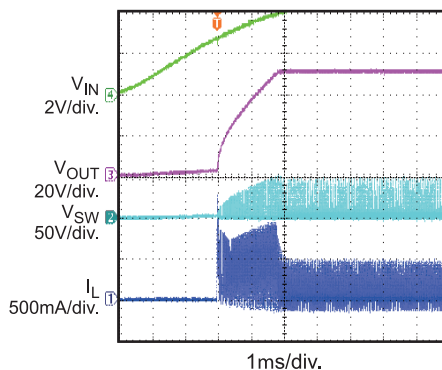
Power Start Up I_{APD}=2.5mA , V_{IN} = 5.5V
