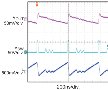
Steady State I_{APD}=2mA , V_{IN} = 4.5V
