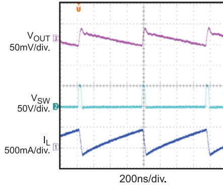
Steady State I_{APD}=2mA , V_{IN} = 2.7V
