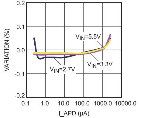
Load Regulation
