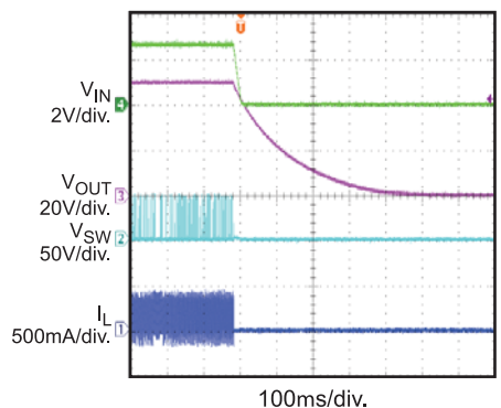
Power Shutdown I_{APD}=2.5mA , V_{IN} = 2.7V
