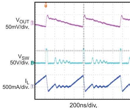
Steady State I_{APD}=2mA , V_{IN} = 5.5V
