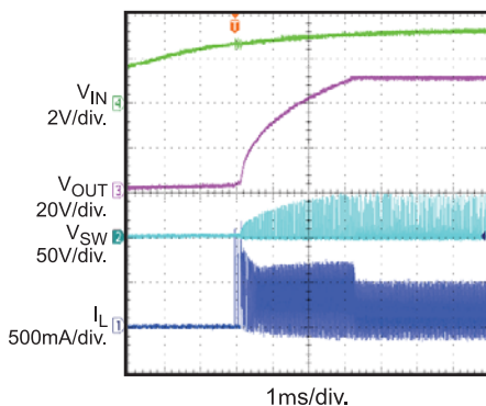
Power Start Up I_{APD}=2.5mA , V_{IN} = 3.3V
