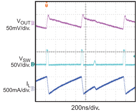
Steady State I_{APD}=2mA , V_{IN} = 3.3V
