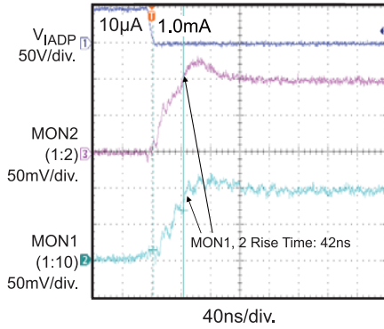
APD Monitor Current Response Speed – 10µA to 1mA Step V_{IN} = 3.3V , V_{OUT} = 50V
