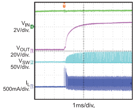
Power Start Up I_{APD}=2.5mA , V_{IN} = 2.7V
