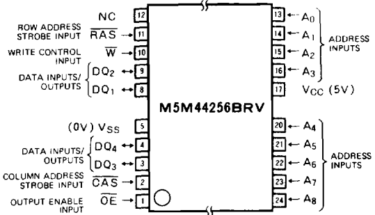
Outline 24P3B-M (TSOP)
