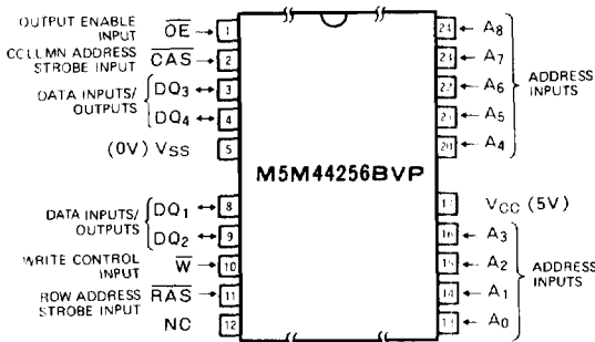
Outline 24P3B-L (TSOP)
