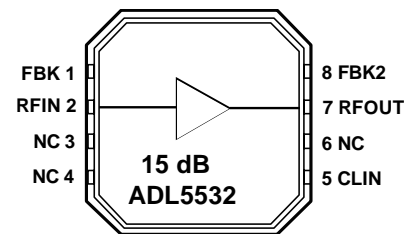
Figure 1. Block Diagram
