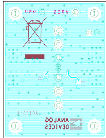
Figure 8. Evaluation Board Layout (Bottom)
