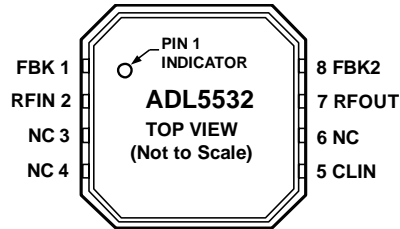
Figure 2. Pin Configuration
