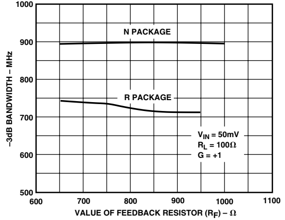
TPC 16. -3 dB Bandwidth vs. R_F , G = +1
