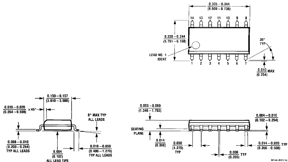
Molded Dual-In-Line Package (M) Order Number DS75107M, DS75107AM NS Package Number M14A
