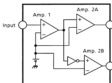
Figure 1 Block diagram
