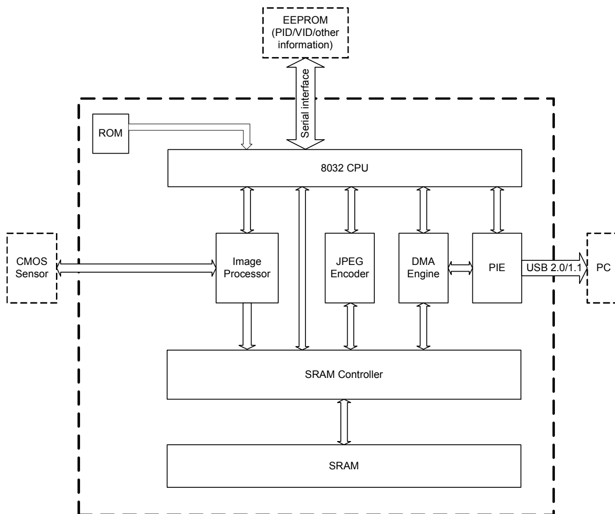
FIGURE 2-1: SQ930C INTERNAL BLOCK DIAGRAM
