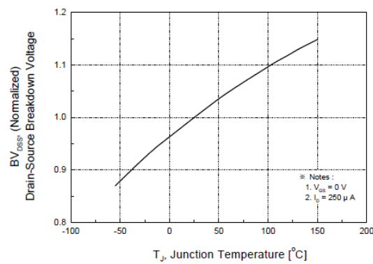
Fig. 3 Breakdown Voltage Variation vs Temperature
