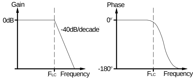
Figure14 - Gain and phase of LC filter
