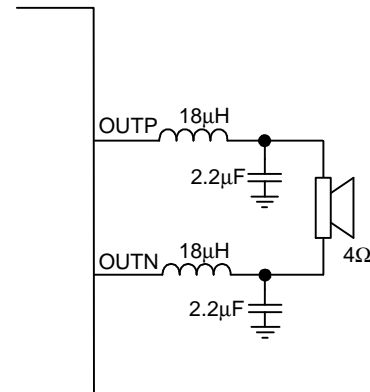
Figure 4. LC output filter for 4Ω speaker
