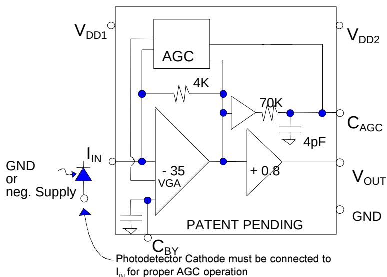
Figure 1: Equivalent Circuit
