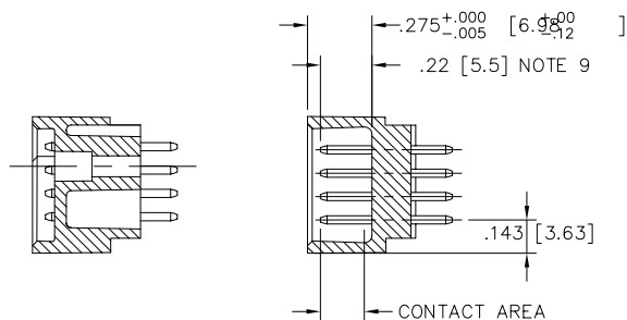
SECTION W-W
