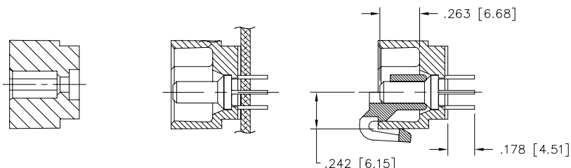
SECTION U-U
