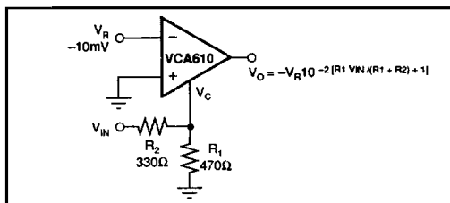
FIGURE 10. Signal Drive of the VCA610 Gain Control Pin Produces and Exponential Response, Re-expanding Signal Compressed by Figure 9.
