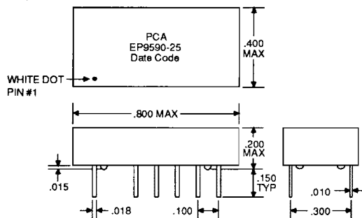
Package Dimensions
