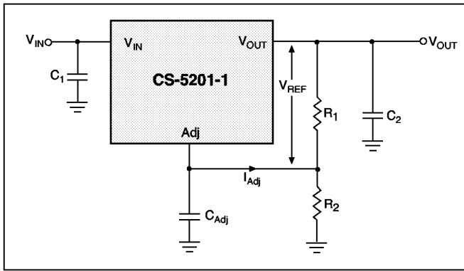
Figure 1. Resistor divider scheme.
