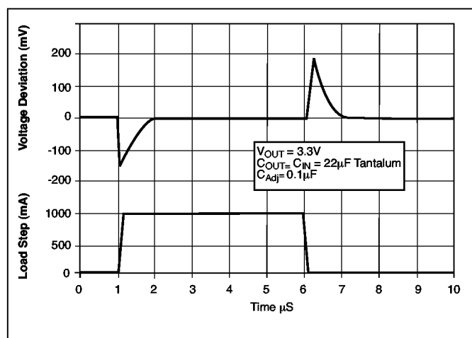
Transient Response
