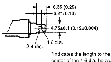
Solder terminal (A) (or quick connect terminals #187 series)
