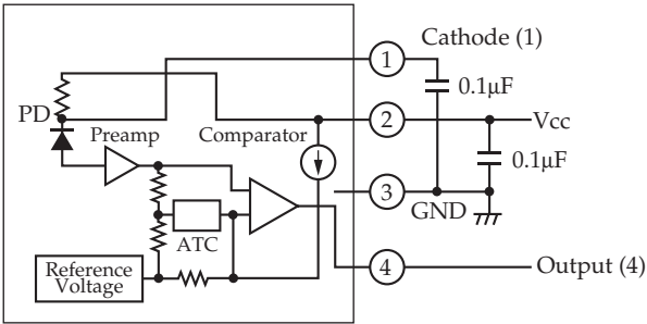
Optical Receiving Module LD-AP1-R2
