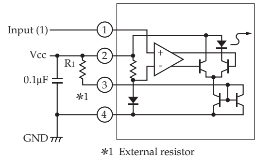
Optical Transmission Module LD-AP1-R1
