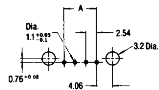
P.C. Board Hole Pattern Layout
