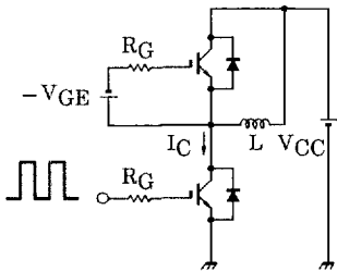
(Note 1) Switching Time Test Circuit & Timing Chart
