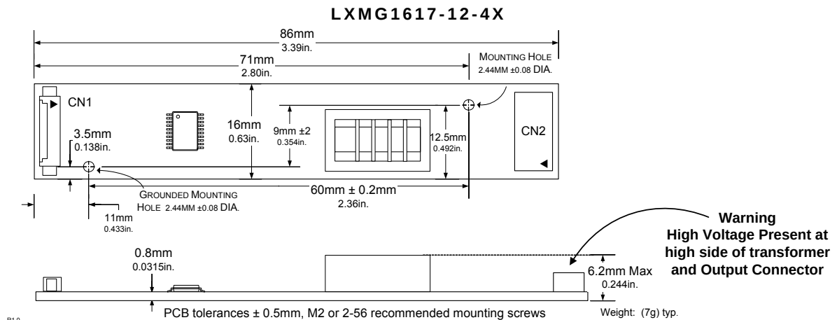
PHYSICAL DIMENSIONS
