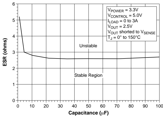
Stability vs ESR
