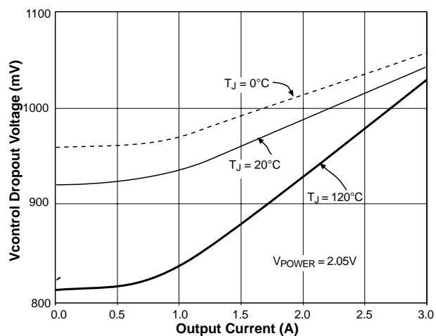
V_{CONTROL} Dropout Voltage vs Output Current
