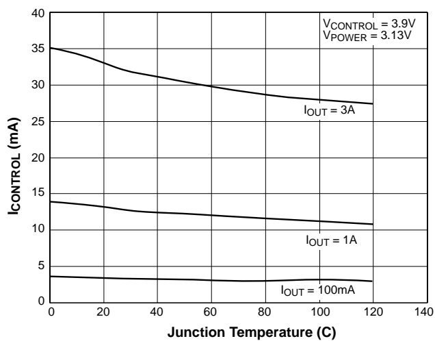
V_{CONTROL} Supply Current vs Junction Temperature
