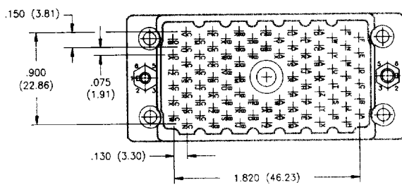
90 PIN PLUG
