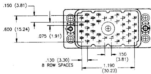
38 PIN PLUG
