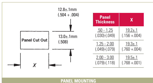
PANEL MOUNTING
