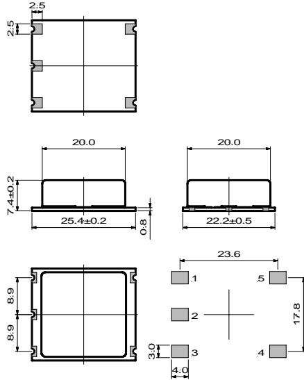
PC board footprint
