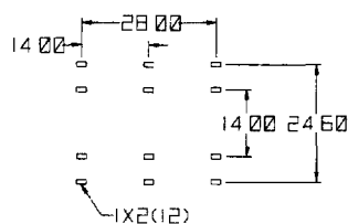
RECOMMENDED PCB LAYOUT (BOTTOM VIEW)
