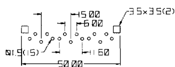
RECOMMENDED PCB LAYOUT (BOTTOM VIEW)
