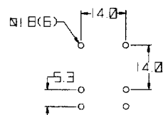
RECOMMENDED PCB LAYOUT (BOTTOM VIEW)
