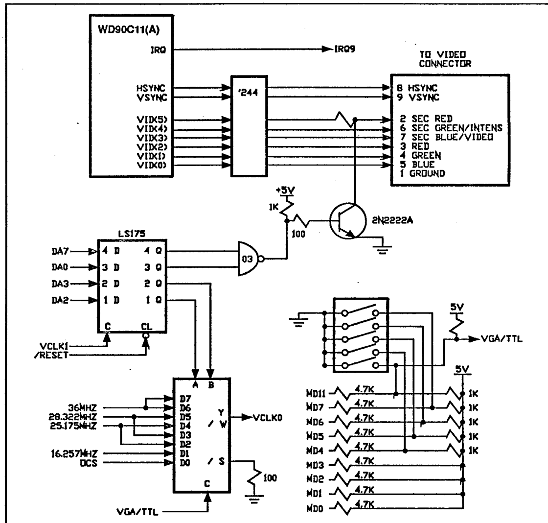
FIGURE A-8. WD90C11(A) AND TTL MONITOR CONNECTIONS
