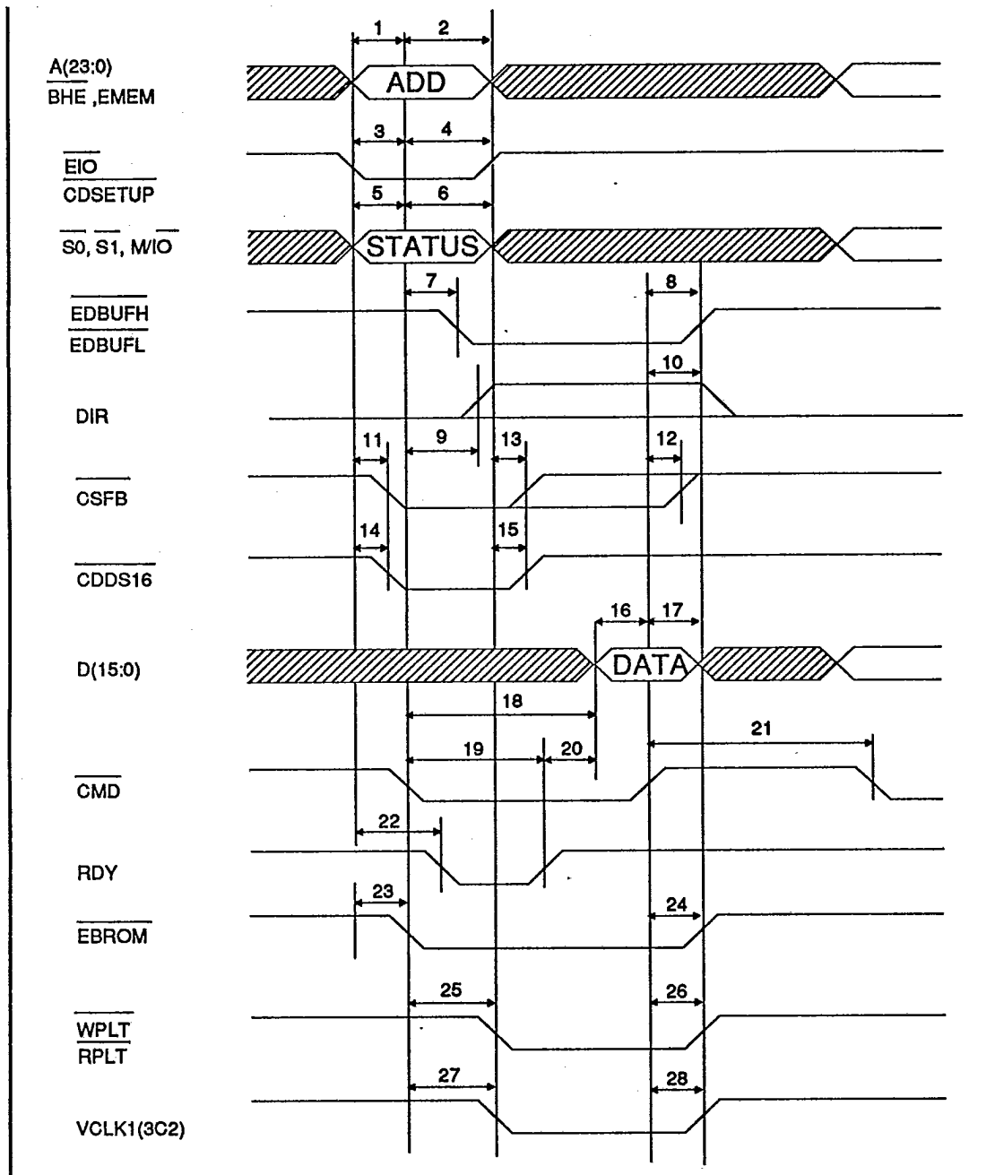
FIGURE 7-4. MICRO CHANNEL MODE BUS TIMING
