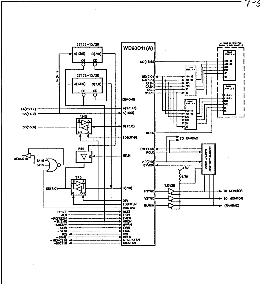
FIGURE A-5. 16-BIT PC AT INTERFACE WITH 16-BIT BIOS (With Optional 512 KBytes: 4- 256K by 4 DRAM)
