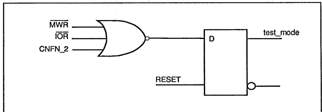
FIGURE C-1. TEST MODE CIRCUIT
