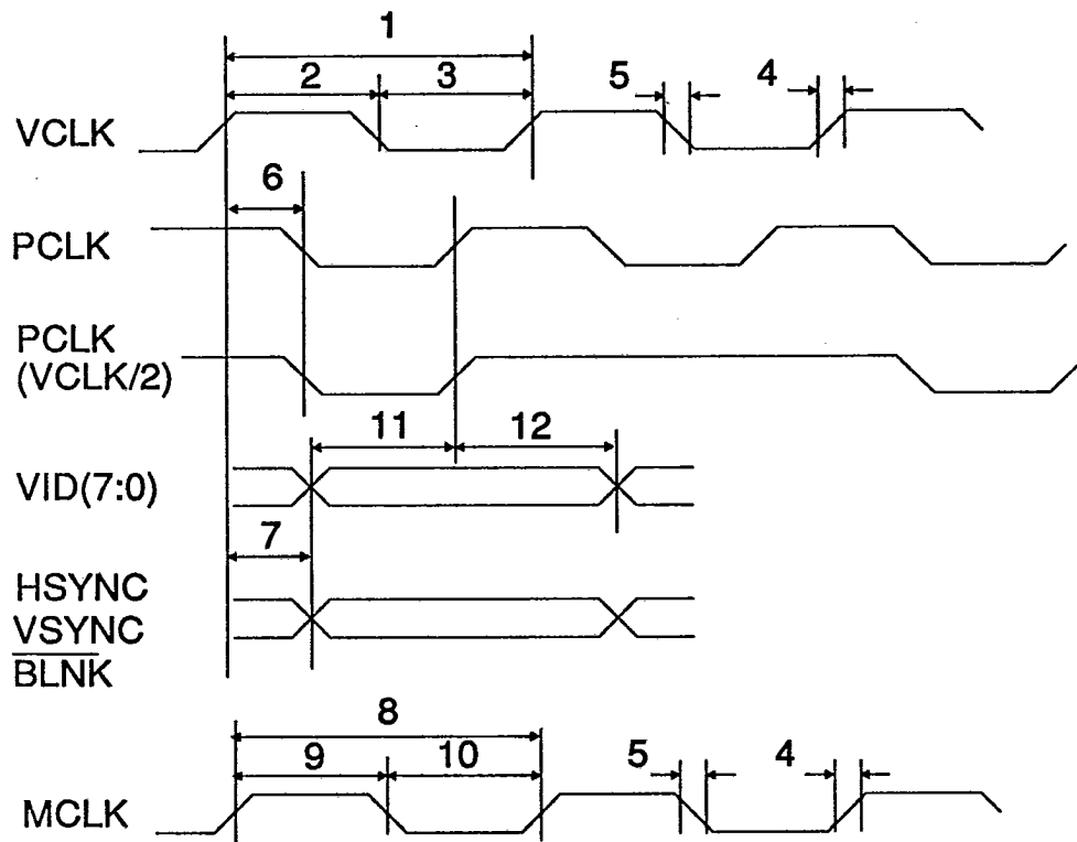
FIGURE 7-2. CLOCK AND VIDEO TIMING
