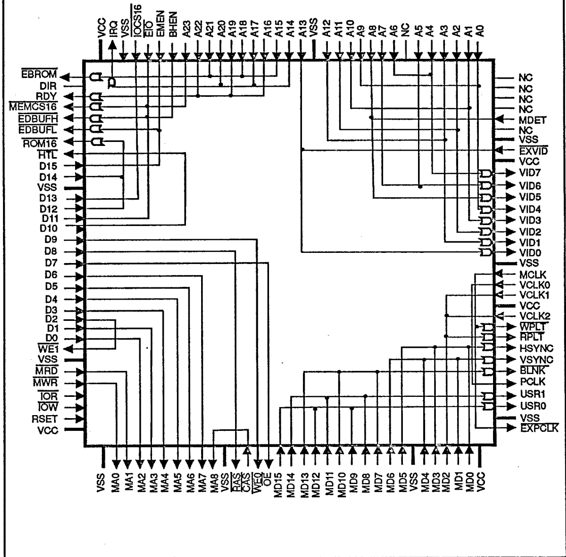
FIGURE C-2. WD90C11A PIN SCAN MAP
