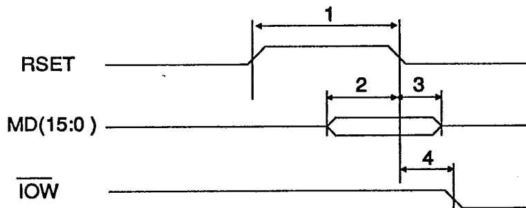
FIGURE 7-1. RESET TIMING
