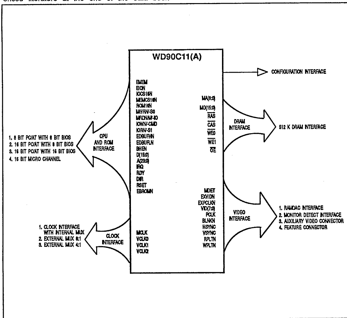
FIGURE A-1. WD90C11(A) INTERFACES
