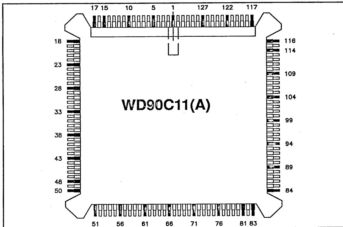
FIGURE 4-1. WD90C11(A) PIN DIAGRAM
