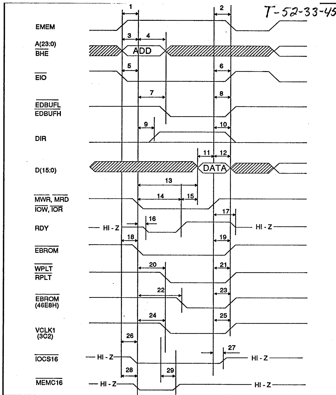
FIGURE 7-3. AT MODE BUS TIMING
