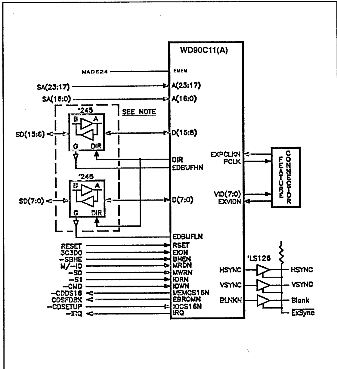
FIGURE A-6. 16-BIT MICRO CHANNEL INTERFACE
