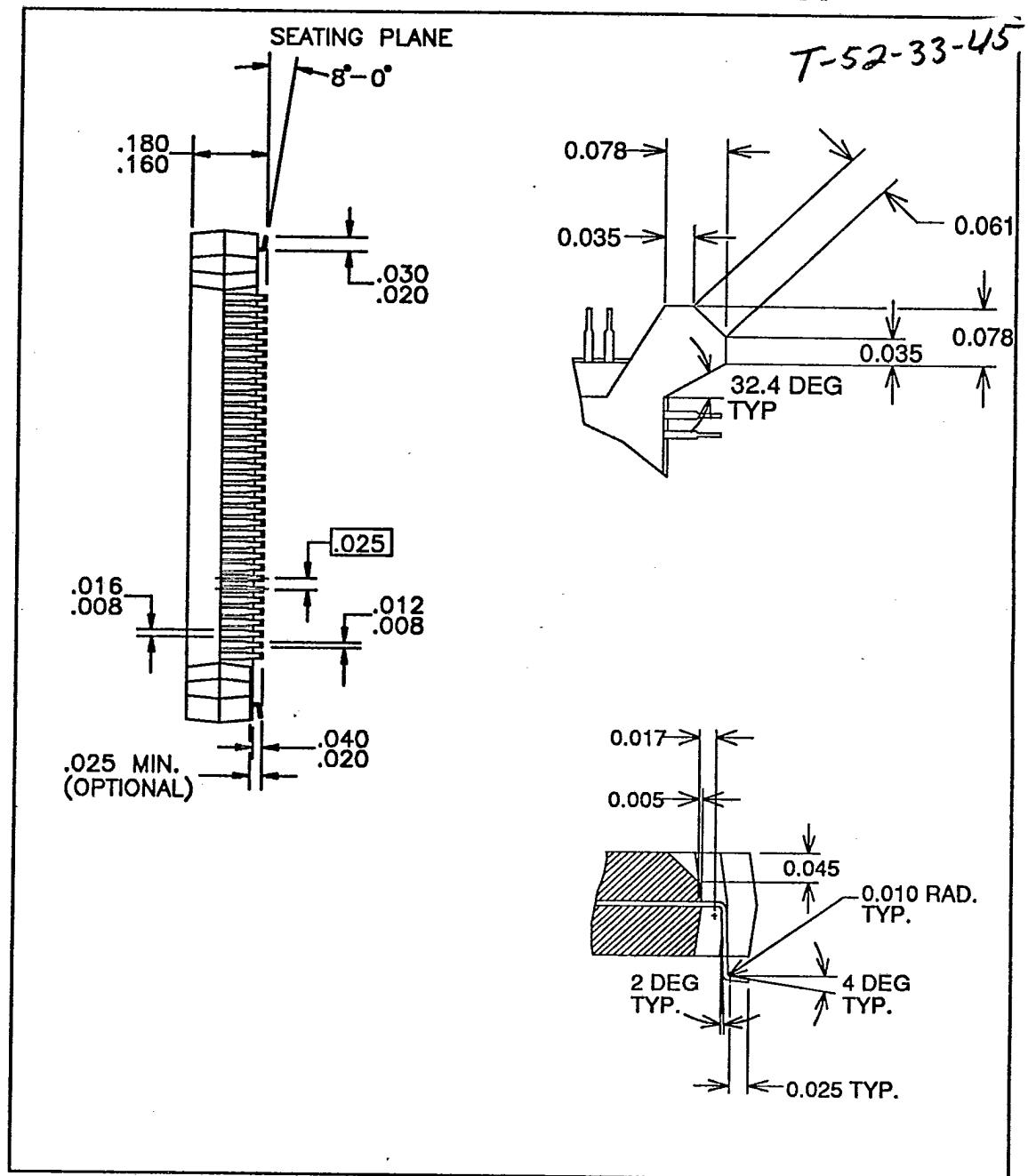
FIGURE 8-2. 132-PIN JEDEC PLASTIC FLAT PACKAGE (PFP)
