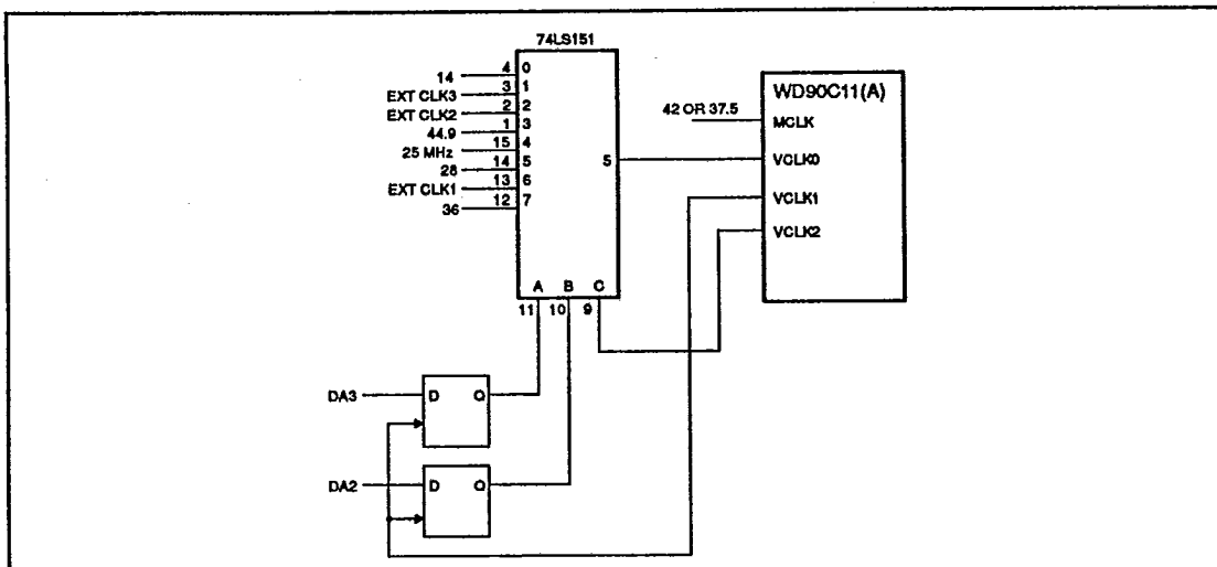
FIGURE A-10. EXTERNAL VIDEO CLOCK MULTIPLEXING
