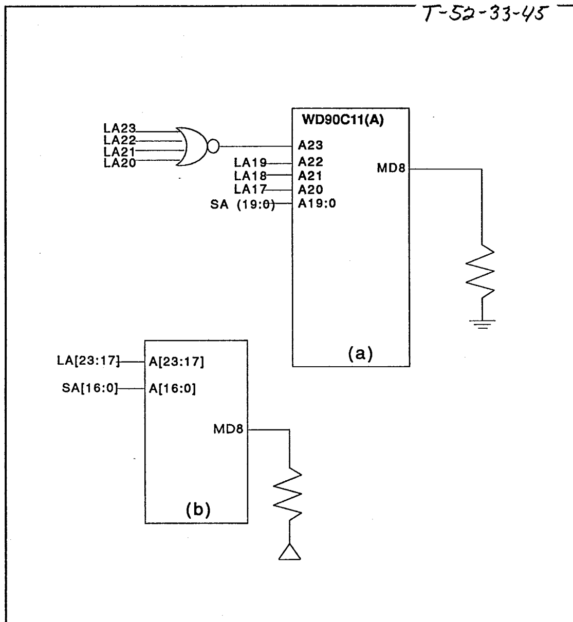
FIGURE A-4. WD90C11(A) INTERFACE FOR 286 OR 386-BASED SYSTEM
