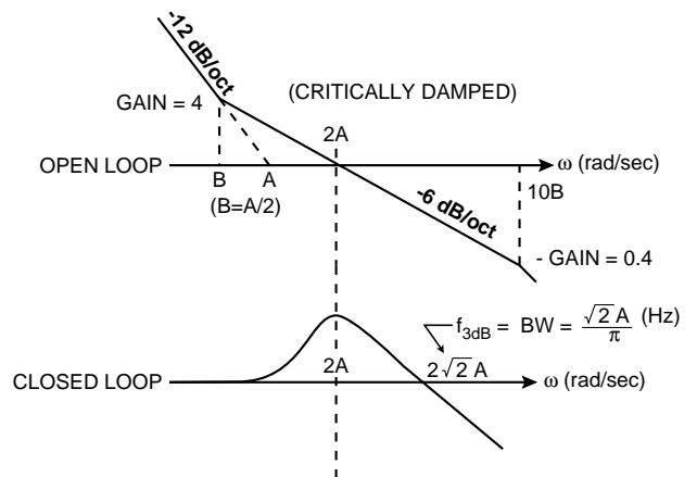
FIGURE 6. BODE PLOTS
