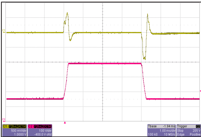
Figure 13: Output voltage response to step-change in input voltage (155V - 400V - 155V) in 250 \mu s. Load cap: 10 \mu F, 100m \Omega ESR tantalum cap and 1 \mu F ceramic cap. Ch 1: Vout (500mV/div). Ch 2: Vin (100V/div)
