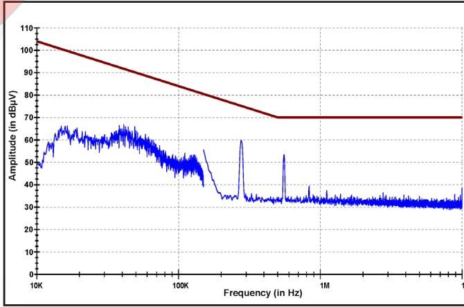
Figure 24: High frequency conducted emissions of MQFL-270-05S, 5V out module at 120W output with MQFL-270-P filter, as measured with Method CE102. Limit line shown is the 'Basic Curve' for all applications with a 270V source.
