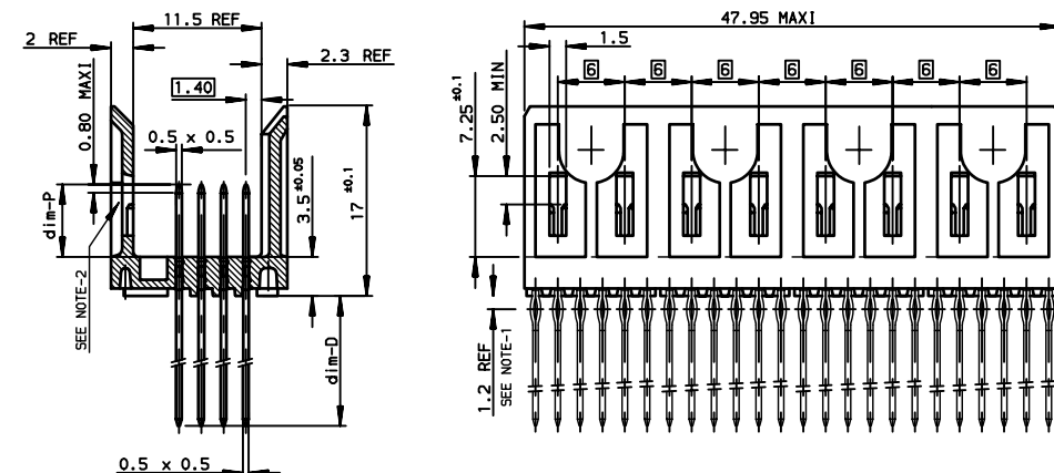
LAYOUT FOR P.C.B (PER 12mm LENGTH)
