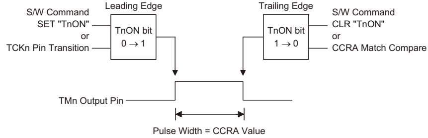
Single Pulse Generation (n = 0)
