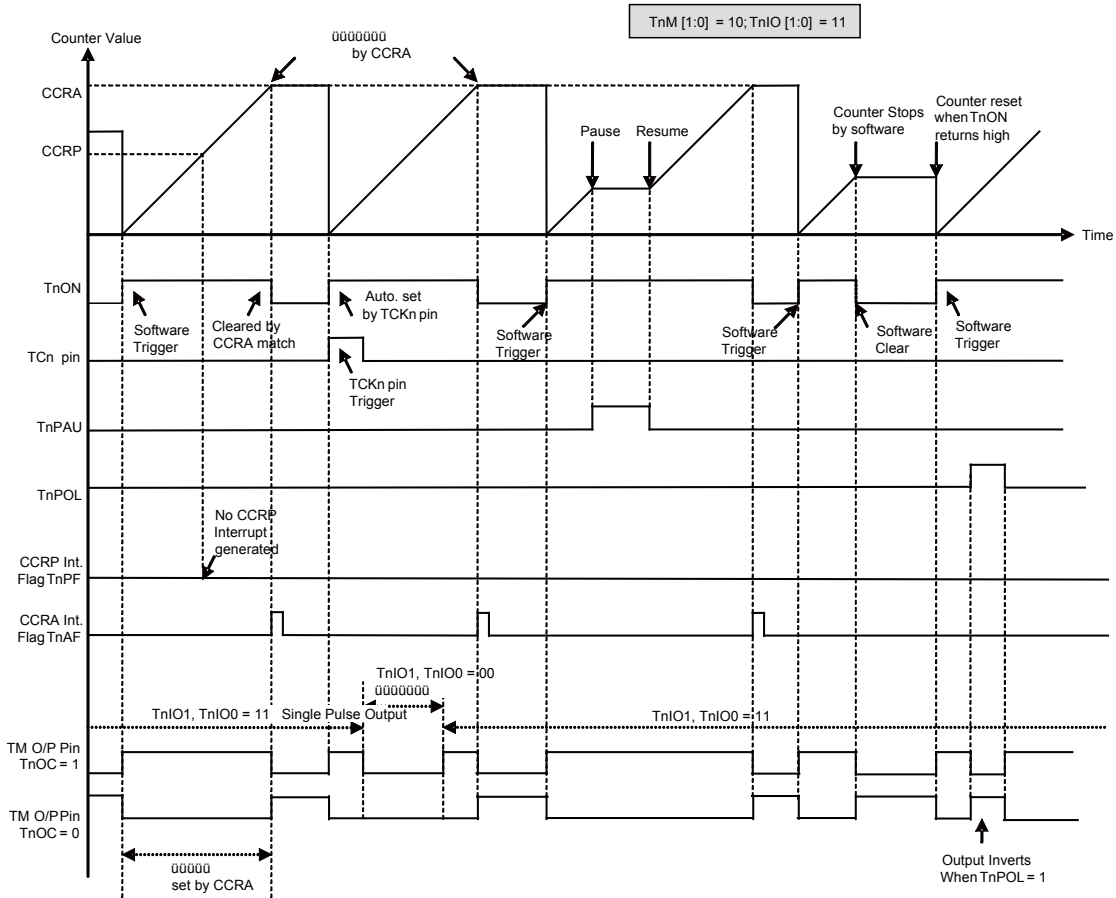
Single Pulse Mode
