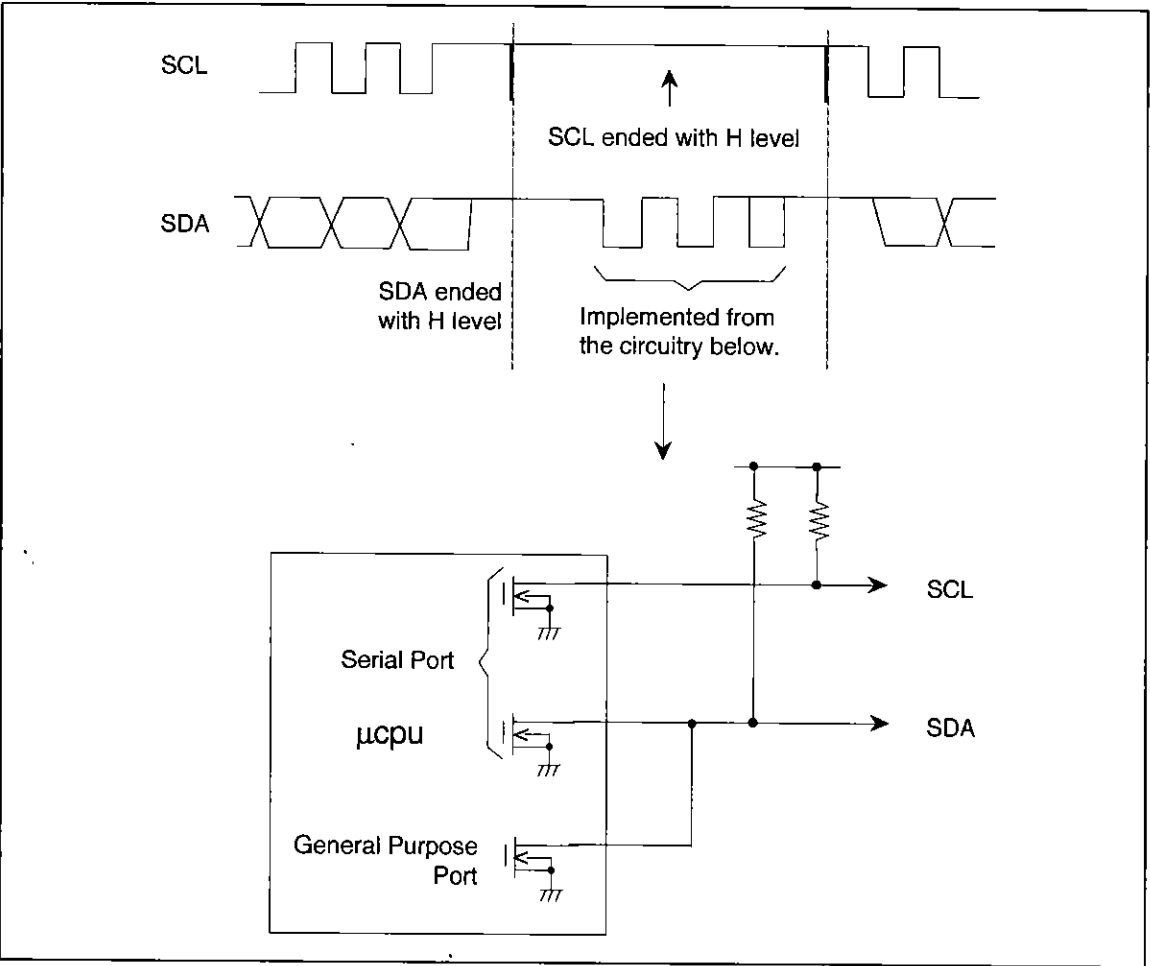
Figure 5 Method 2
