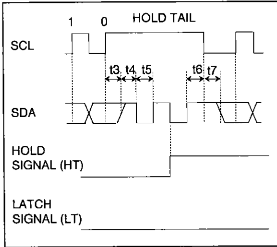
Figure 2 HOLD Mode
