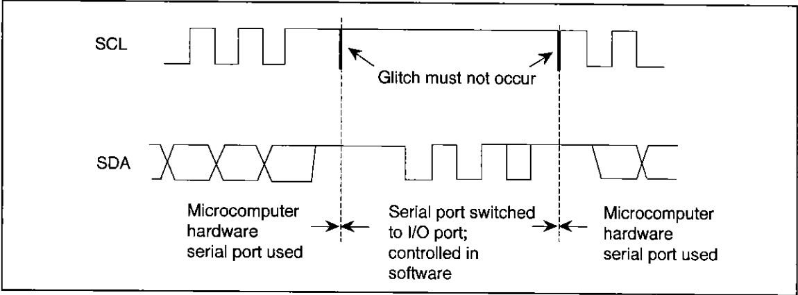
Figure 4 Method 1
