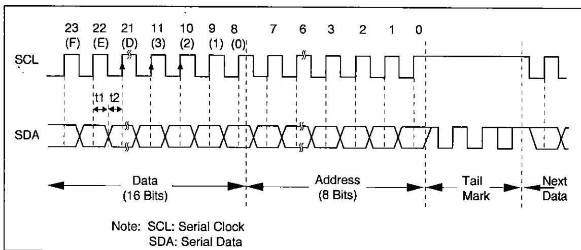
Figure 1 Timing Chart
