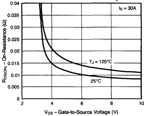
Fig. 6 – On-Resistance vs. Gate-to-Source Voltage
