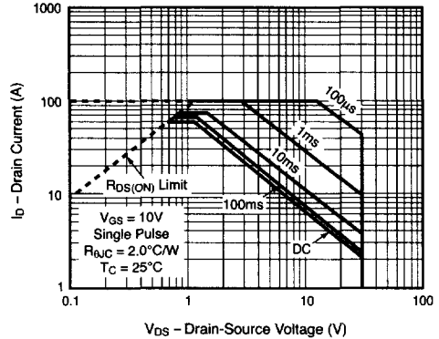
Fig. 13 – Maximum Safe Operating Area
