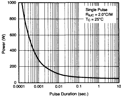
Fig. 12 – Power vs. Pulse Duration
