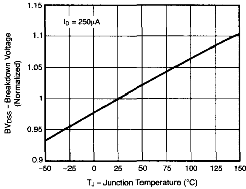
Fig. 10 – Breakdown Voltage vs. Junction Temperature
