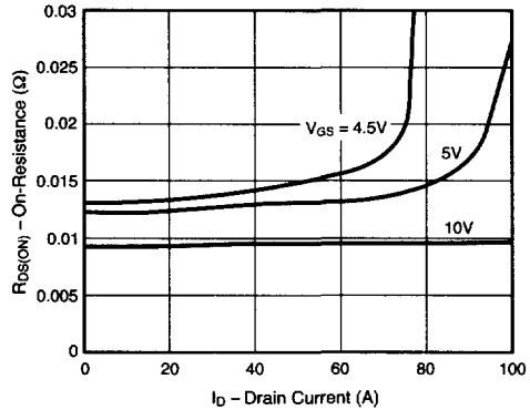
Fig. 4 – On-Resistance vs. Drain Current
