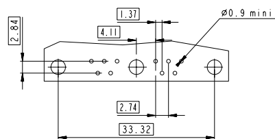
LAYOUT AND CONNECTOR DIMENSIONS
