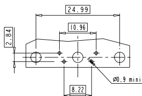
LAYOUT AND CONNECTOR DIMENSIONS
