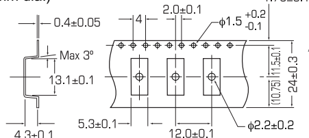
1,000 pcs. per reel (330mm dia.)
