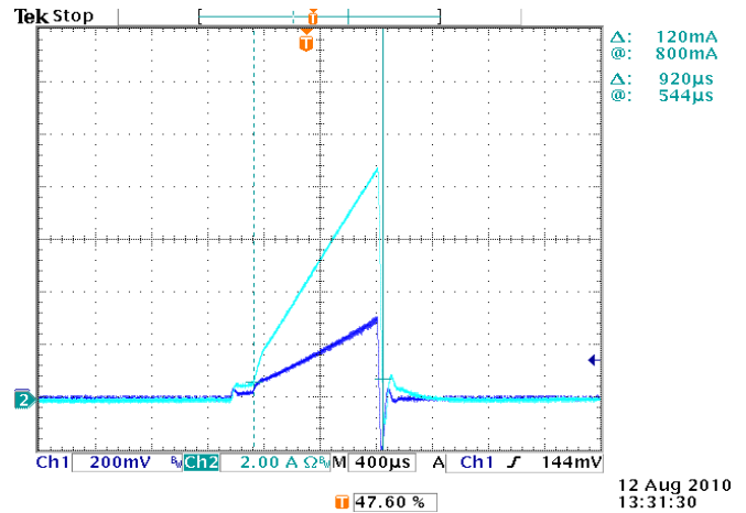
CH1: Output voltage waveform CH2: Output current waveform Test condition: 48V input with a Rout (0.171ohm) Expansion of on time portion of above figure
