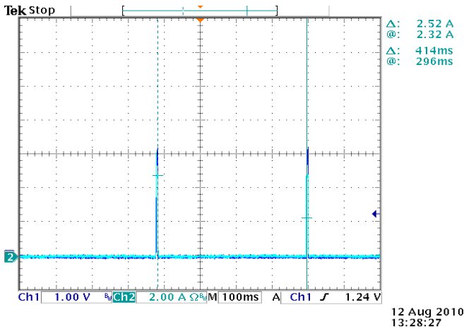
CH1: Output voltage waveform CH2: Output current waveform Test condition: 48V input with a Rout (0.171ohm)
