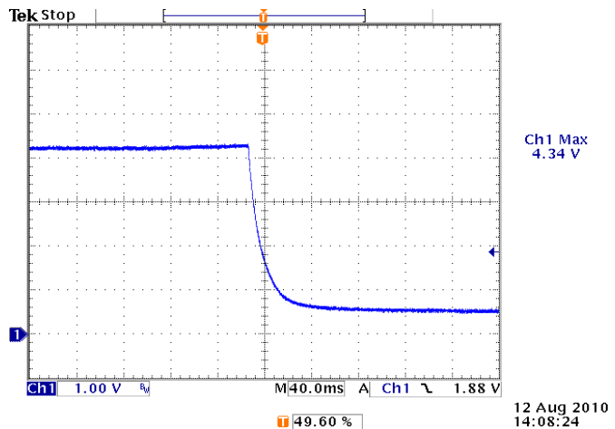
CH1: Output voltage waveform
