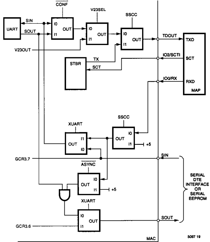
Figure 5a. MAC II Internal Data Path
