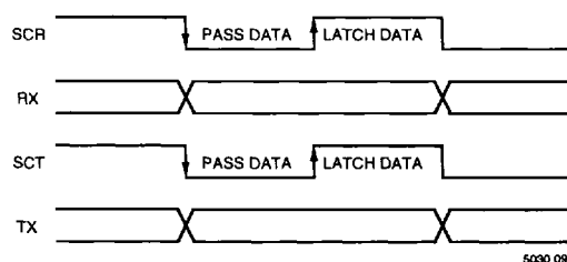
(a) Signal Interface with MAP, (Synchronous mode)
